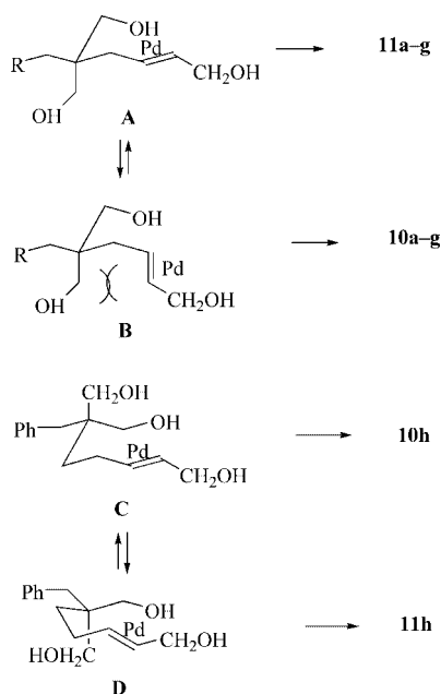
Figure 3. Models for Pd II -catalyzed cyclization.
