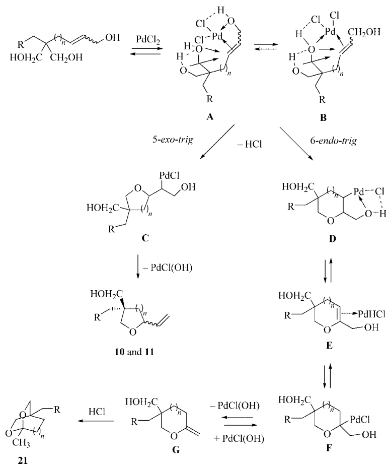
Scheme 7. Mechanism of the Pd II -catalyzed cyclization.
