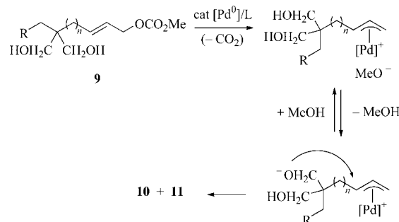
Scheme 5. Mechanism of the Pd 0 -catalyzed cyclization.
