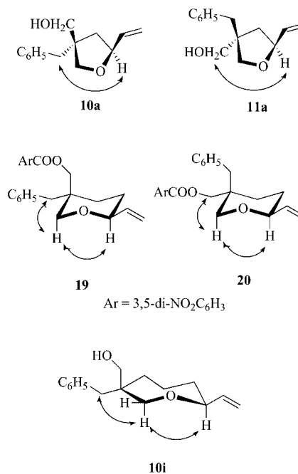
Figure 1. Observed NOE effects.
