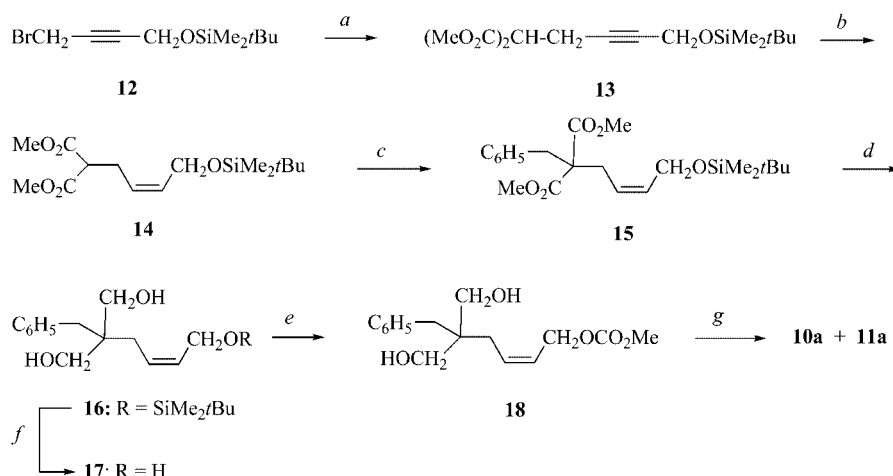
Scheme 4. Synthesis of dihydroxycarbonate 18 and Pd-catalyzed cyclization; reagents and conditions: (a) CH_2(CO_2Me)_2 , NaH, THF, DMF, reflux, 5 h, 85%; (b) H_2 , 1 bar, Pd Lindlar, cyclohexane, ethyl acetate, room temp., 48 h, 98%; (c) NaH, C_6H_5CH_2Br , THF, DMF, reflux, 5 h, 96%; (d) AlH_4Li , Et_2O , 0^\circ C \rightarrow room temp., 0.5 h, 73%; (e) Bu_4NF \cdot 3H_2O , THF, room temp., 15 h, 75%; (f) ClCO_2CH_3 , C_5H_5N , CH_2Cl_2 , 0^\circ C \rightarrow room temp., 2 h, 54%; (g) Pd_2(dba)_3 , ligand, THF, 1 h, room temp.
