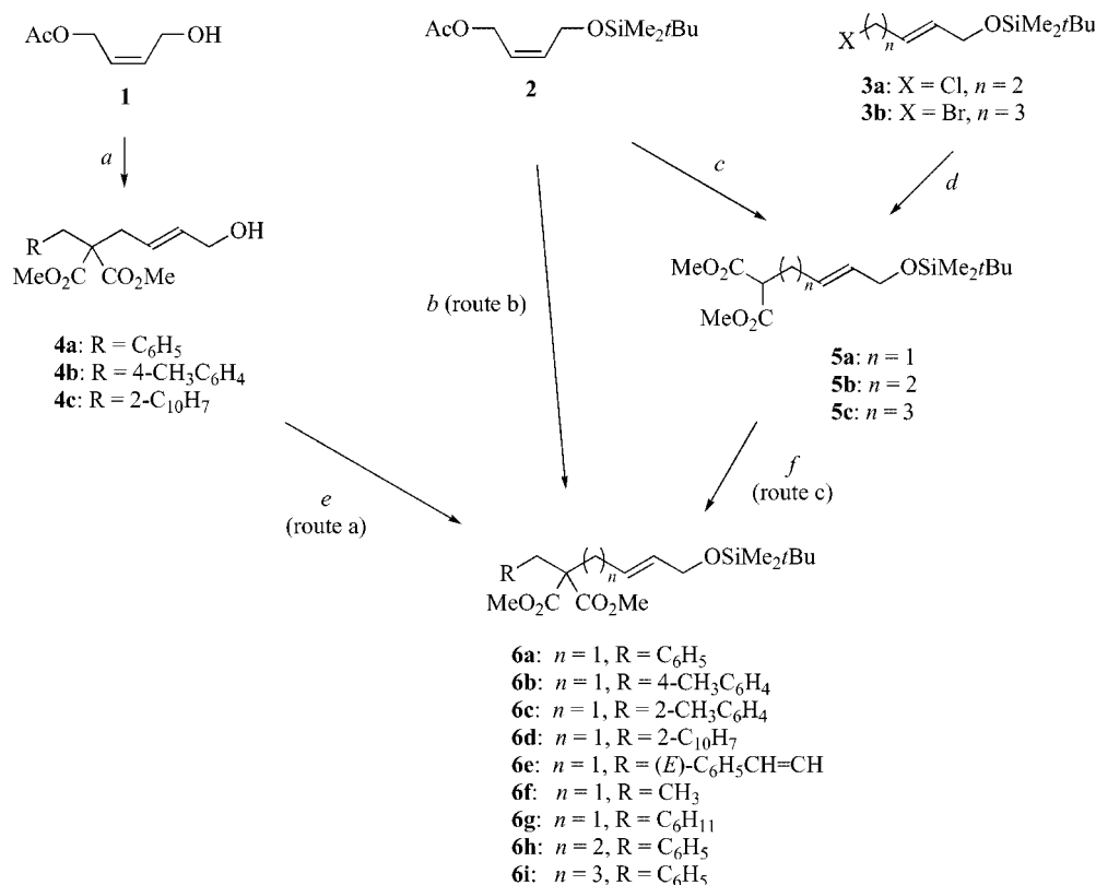
Scheme 2. Synthesis of silylated dimethyl malonates 6a–i ; reagents and conditions: (a) (i) Pd 2 (dba) 3 , dppb, THF, room temp., 0.5 h; (ii) RCH 2 CH(CO 2 Me) 2 (R = C 6 H 5 , 4-CH 3 C 6 H 4 , or 2-C 10 H 7 ), NaH, THF; (iii) 1 , THF, room temp., 24 h; (b) (i) Pd 2 (dba) 3 , dppb, THF, room temp., 0.5 h; (ii) RCH 2 CH(CO 2 Me) 2 (R = ( E )-C 6 H 5 CH=CHCH 2 , CH 3 , or C 6 H 11 ), NaH, THF; (iii) 2 , THF, room temp., 24 h; (c) (i) Pd 2 (dba) 3 , dppb, THF, room temp., 0.5 h; (ii) CH 2 (CO 2 Me) 2 , NaH, THF, DMF, reflux, 5 h; (e) t BuMe 2 SiCl, imidazole, Et 3 N, CH 2 Cl 2 , room temp., 15 h; (f) (i) 5 , NaH, THF, DMF, room temp., 0.5 h; (ii) RCH 2 Br (R = C 6 H 5 , or 2-CH 3 C 6 H 5 ), reflux, 5 h.
