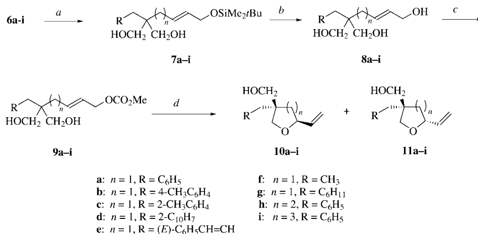
Scheme 3. Synthesis of dihydroxycarbonates 9a-i and Pd-catalyzed cyclization to oxygen heterocycles 10 and 11 ; reagents and conditions: (a) AlH_4Li , Et_2O , 0^\circ C \rightarrow room temp., 0.5 h; (b) Bu_4NF \cdot 3H_2O , THF, room temp., 15 h; (c) ClCO_2CH_3 , C_5H_5N , CH_2Cl_2 , 0^\circ C \rightarrow room temp., 2 h; (d) Pd_2(dba)_3 , ligand, THF, 1 h, room temp.
