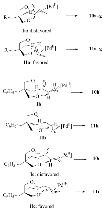
Figure 2. Models for Pd 0 -catalyzed cyclization.
